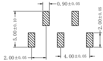
Recommended PCB Layout SM1 Type
