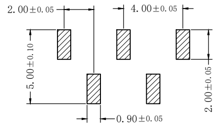
Recommended PCB Layout SM2 Type
