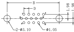
P. C BOARD LAYOUT (15PIN) GENERAL TOLERANCE: ±0.05
