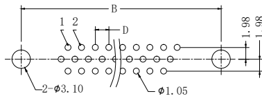
P. C BOARD LAYOUT (26~62PIN) GENERAL TOLERANCE: ±0.05
